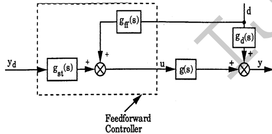
Fig. 3 Feed forward control system
